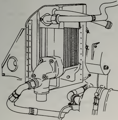
FIGURE 6-18. Oil cooler.
